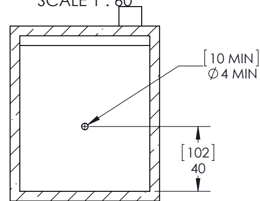
SECTION F-F
